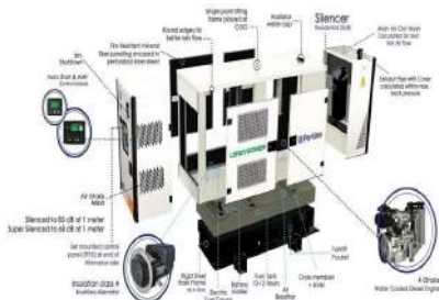
ATP ENCLOSURE/CANOPY
